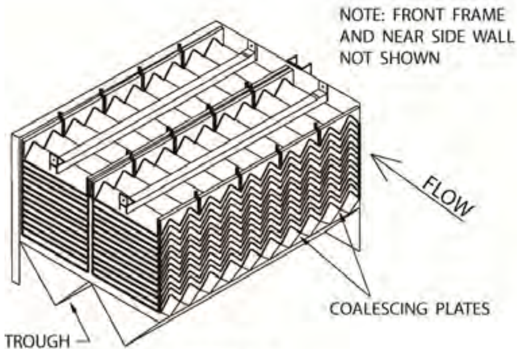
FIGURE 3 PROPOSED INSTALLATION COALESCING PACK MODULE
