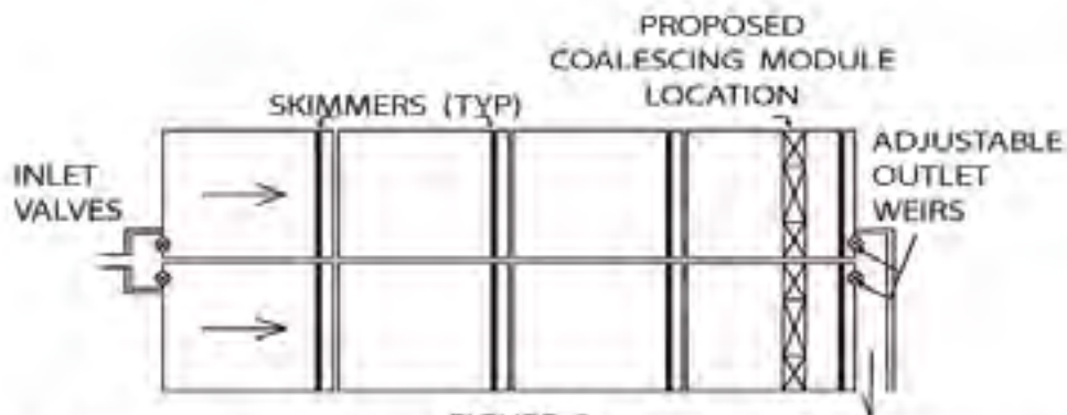
FIGURE 2 PROPOSED CONFIGURATION WITH COALESCING PLATES ADDED
