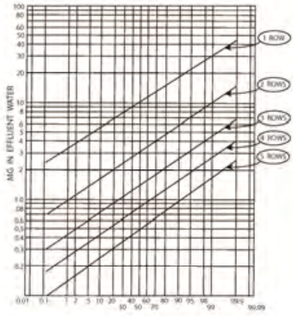
FIGURE 4 PROBABILITY OF EFFLUENT BEING LESS THAN INDICATED AT 15,000 L/D TOTAL FLOW
