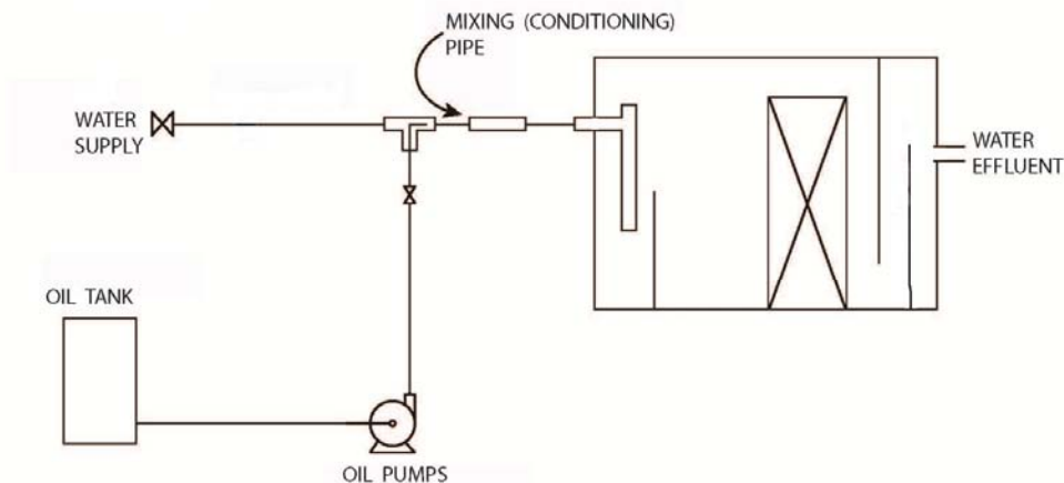
FIGURE 1 SCHEMATIC OF FLOWS DURING TEST
